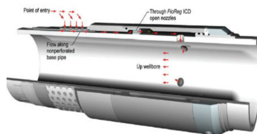
Figure 1: Nozzle type ICD
