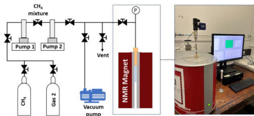
Figure 1: Experimental Setup
