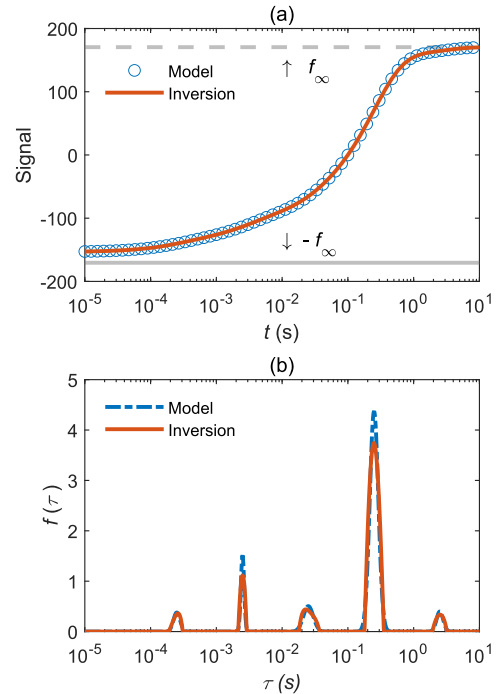
Fig. 1: Excellent agreement was found between the model and its inversion for non-ideal cases; here with recovery factor \alpha = 1.9 and a signal that is still rising at the longest measurement times.
