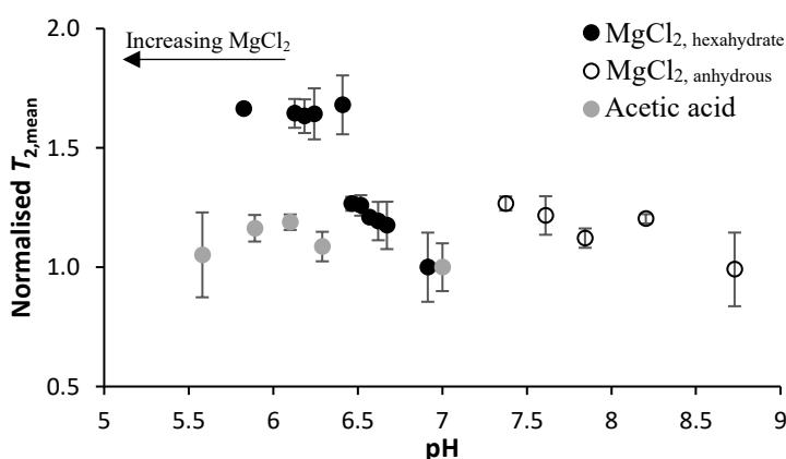
Fig. 1: Normalised T_{2,\text{mean}} as a function of pH for tailings mixed with \text{MgCl}_2 ,hexahydrate, \text{MgCl}_2 ,anhydrous and acetic acid solutions. Concentration of \text{MgCl}_2 ranges from 0.5M to 2.5M.
